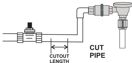
Standard Coupling - High Flow / Sprinkler Only
