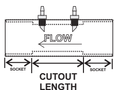
Standard Coupling - High Flow / Sprinkler Only
