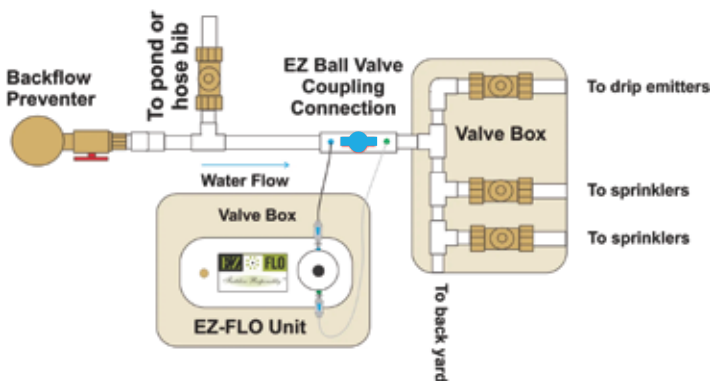
TYPICAL MULTI ZONE INSTALLATION
